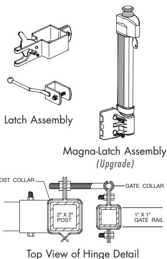
SINGLE GATE (2110 FLAT TOP) INSTALLATION DETAIL
