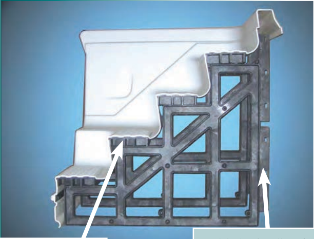
Modular bracing allows for optional deck support.
